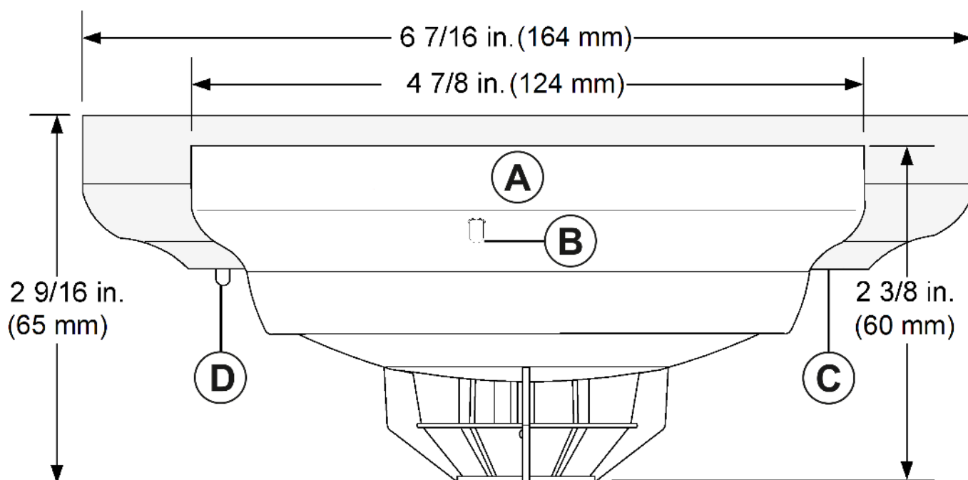
Figure 4: Dimensions
